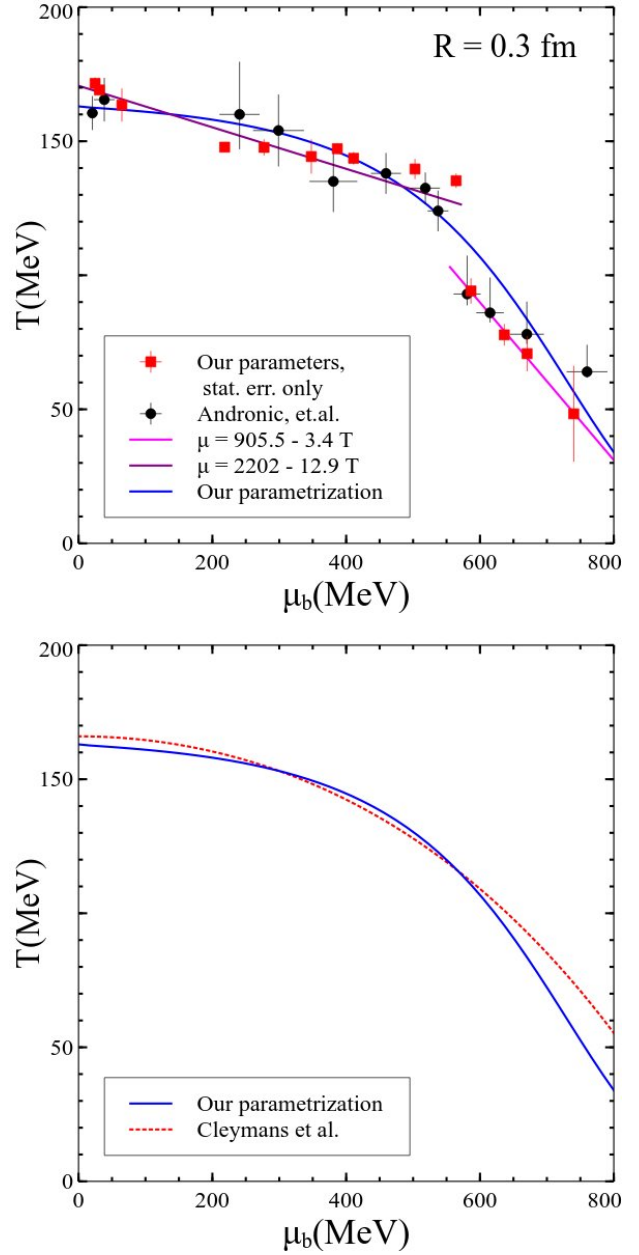
Fig. 1. Chemical freeze out temperature dependence on the baryonic chemical potential \mu_b . The symbols in the upper panel correspond to the fit of hadron yield ratios obtained in [2] (squares) and in [3] (circles) for the same value of the hard core radius of all hadrons R = 0.3 fm. The solid curve in the upper panel is a fit to the results of [2] and [3] by Eq. (2). The dashed and solid curves in the lower panel correspond to Eqs. (1) and (2), respectively. In fact, the straight lines with the parameters specified in the upper panel describe well the \mu_b dependence of the chemical freeze out temperature
