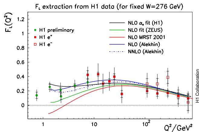
Fig. 2. F_L values from the H1 collaboration
