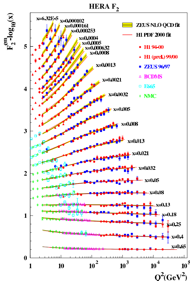
Fig. 1. F_2^{\text{e.m}} measured by the H1 and ZEUS collaborations
