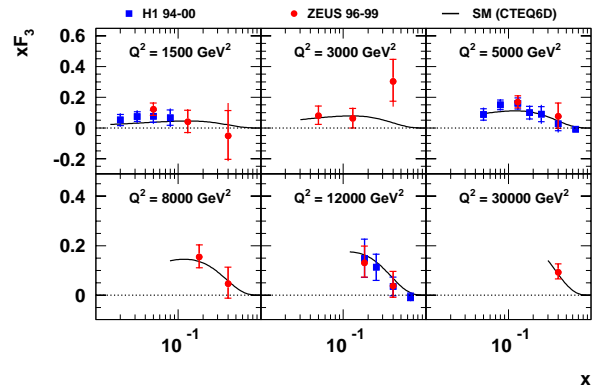
Fig. 5. The xF_3 structure function from the H1 and ZEUS collaborations
