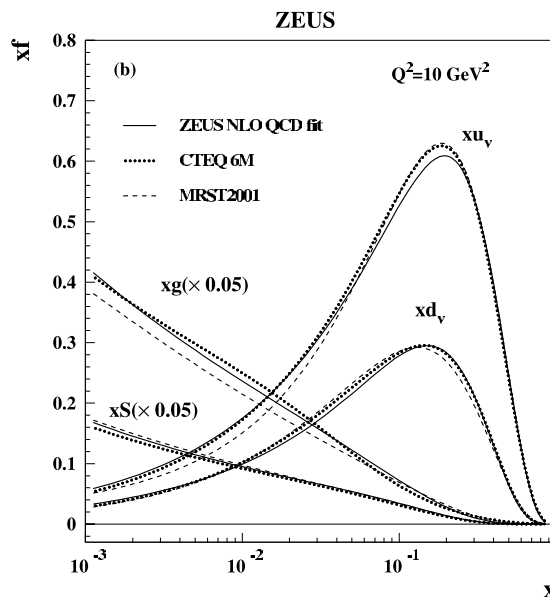
Fig. 7. Parton distribution functions extracted from the ZEUS NLO QCD fit
